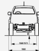
REAR VIEW SINGLE CAB CHASSIS
