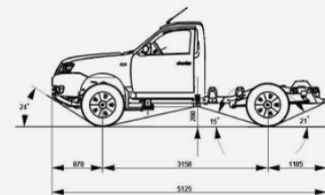
SIDE VIEW SINGLE CAB CHASSIS
