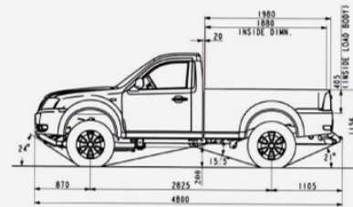
SIDE VIEW SINGLE CAB
