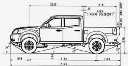
SIDE VIEW DOUBLE CAB
