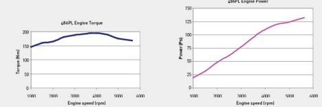
Power & Torque Curve for 2.0L & 3.0L DICOR Engine (Diesel)
