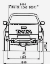
REAR VIEW (DOUBLE CAB / SINGLE CAB)
