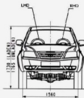
FRONT VIEW (DOUBLE CAB / SINGLE CAB)
